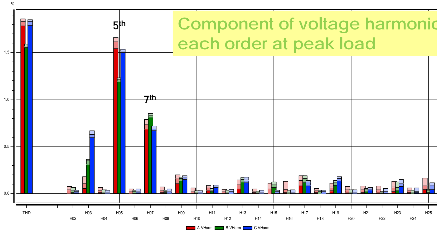
Waveform harmonics
